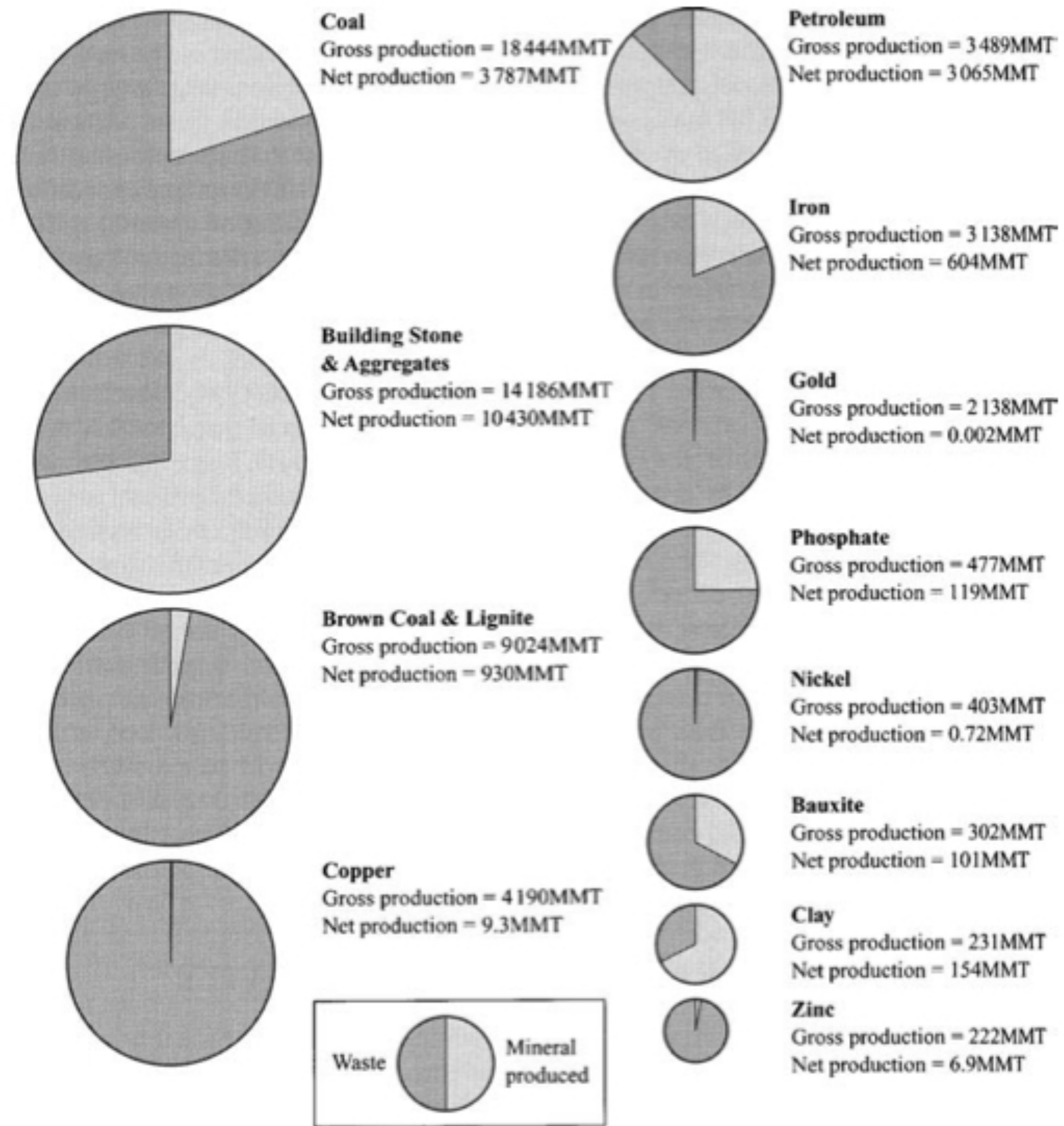
Figure 2 World mineral production and total hidden flows for 12 commodities. MMT, million metric tonnes. From Reference 10.
