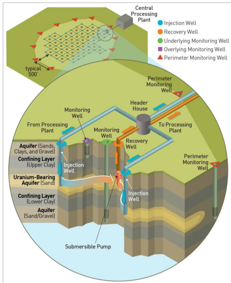
Figure 36 : Schéma de principe de la lixiviation in situ | Nuclear Regulatory Commission · 2017 · cc by 2.0 107
